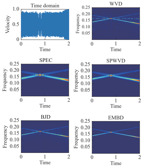
图 6 二分量啁啾信号振动时域图及其时频分布 Fig. 6 Time domain and time frequency distribution of two component chirps vibration
