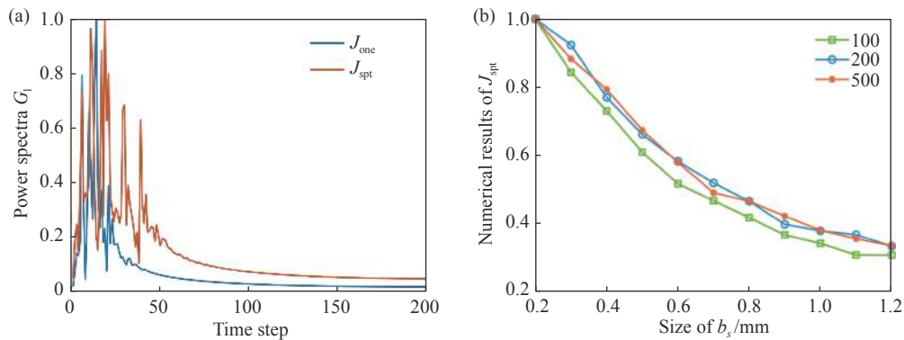
图 6 (a)单通道获得的时间频谱和 4 通道获得的时间空间频谱。(b)四通道获得的归一化评价因子随目标光斑尺寸的变化 Fig. 6 (a) Temporal spectrum obtained by a single-channel, and the spatio-temporal spectrum obtained by a four-channel. (b) The normalized speckle-metric obtained by the four-channel varying with the target spot size
