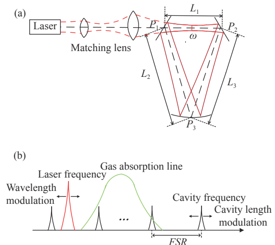
图 12 (a)三角腔横模匹配示意图;(b)纵模匹配示意图 Fig. 12 (a) Schematic diagram of triangular cavity transverse mode matching; (b) schematic diagram of longitudinal mode matching
