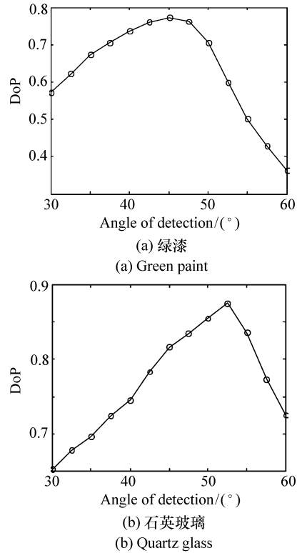
图3 偏振度随探测角度的变化曲线 Fig. 3 DOP curves response with the detection angle
