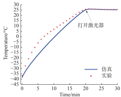
图 13 低温环境下实验测量温度数据与仿真结果对比 Fig. 13 Comparison of the measured temperature and the simulation data in the low temperature environment
