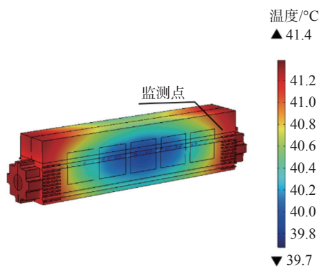
图 7 高温环境下,基于温控制冷的激光器温度分布 Fig. 7 Temperature distribution of laser based on temperature control cooling in high temperature environment
