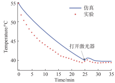
图 12 高温环境下实验测量温度数据与仿真结果对比 Fig. 12 Comparison of the measured temperature and the simulation data in high temperature environment
