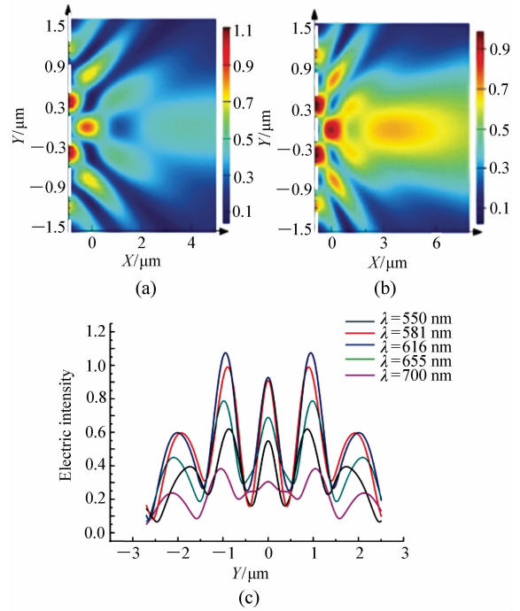
Fig. 8 (a) Near field diffraction of the incident light at 625 nm Corresponding to Fig. 7 (a); (b) near field diffraction of the incident light at 625 nm Corresponding to Fig. 7 (b); (c) curve of near field diffraction of the incident light at 550 – 700 nm corresponding to Fig. 7 (b). White dashed line in the figure (left side) represents the grating location
