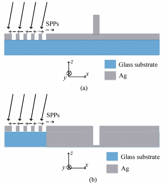
Fig. 7 Schematic diagrams of two kinds of diffraction gratings
