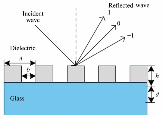
Fig. 1 Cross section of rectangular metal gratings in one-dimension
