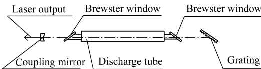
图 1 一级振荡、一级输出 CO 2 激光器谐振腔 Fig. 1 First-order oscillating and first-order output CO 2 laser cavity
