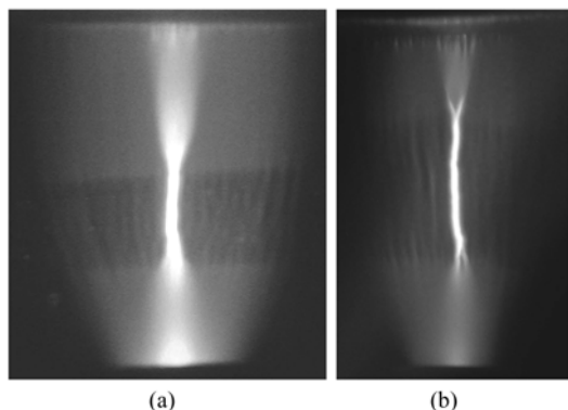
Fig. 3 Photograph of SSVD in mixture C_2H_6:SF_6:Ne = 1:5:5 , W_{el} = 0.2 \text{ J/cm}^3 , T_g = 1\ 250 \text{ K} , \tau_{dis} = 270 \text{ ns} and p = 4.4 \text{ kPa} (a); pure SF_6 , T_g = 1\ 100 , \tau_{dis} = 150 \text{ ns} , W_{el} = 0.11 \text{ J/cm}^3 and p = 2.0 \text{ kPa} (b).
