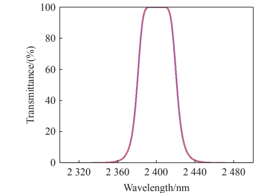
图 15 2400-40 nm 窄带设计曲线 Fig. 15 narrowband design curve of 2400-40 nm
