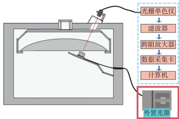
图 3 新直控式光学膜厚监控系统结构简图 Fig. 3 Structural Schematic of the Proposed Direct-Monitoring Optical Film Thickness System
