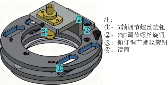
图 14 五自由度光纤装调机构 Fig. 14 Five-Degree-of-Freedom (5-DOF) Fiber Alignment Mechanism
