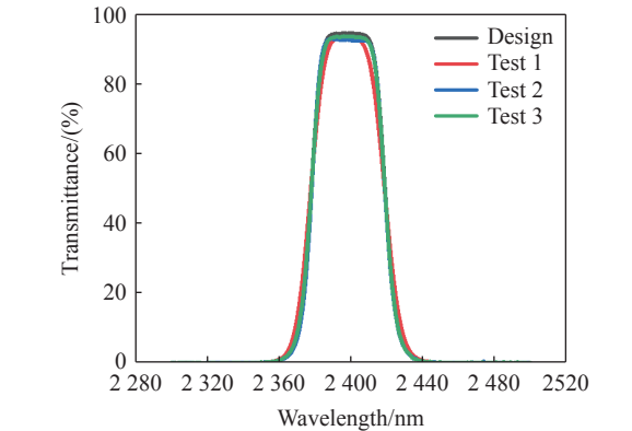
图 18 2400 nm 窄带滤光膜光谱 Fig. 18 Spectrum of 2400 nm narrowband filter film
