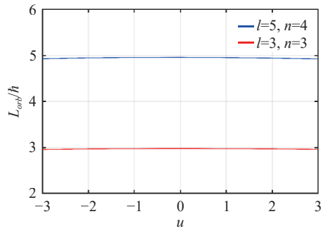
Fig. 6 The OAM at z = 0 versus directional factor of u in x direction at v=3 .
